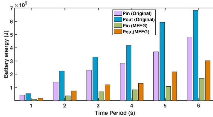
Figure 12: Battery's power
