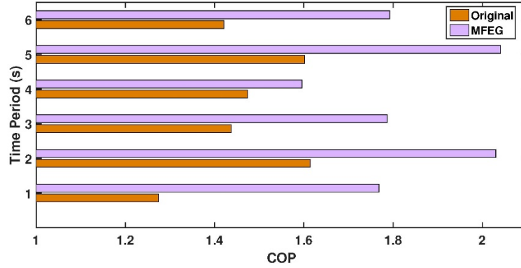
Figure 11: CoP chart
