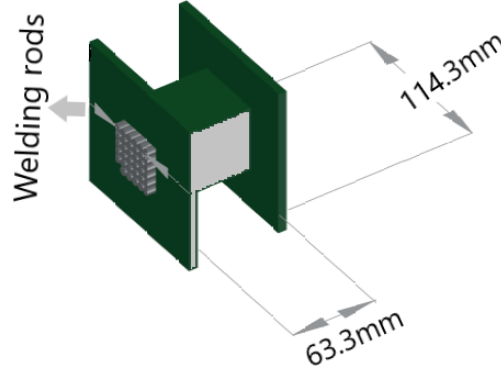
Figure 6: MFE's Spool
