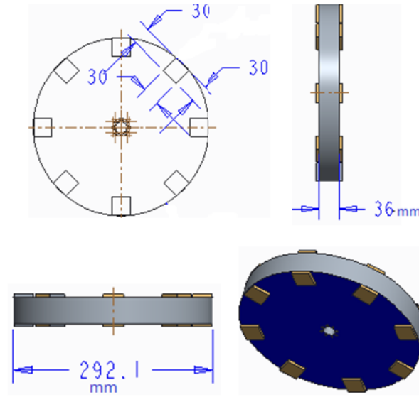
Figure 3: Rotor design
