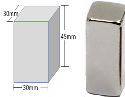
Figure 4: Neodymium magnet's dimensions
